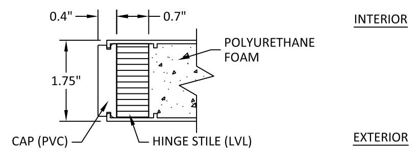
3 6 HORIZONTAL SECTION INSWING/OUTSWING
