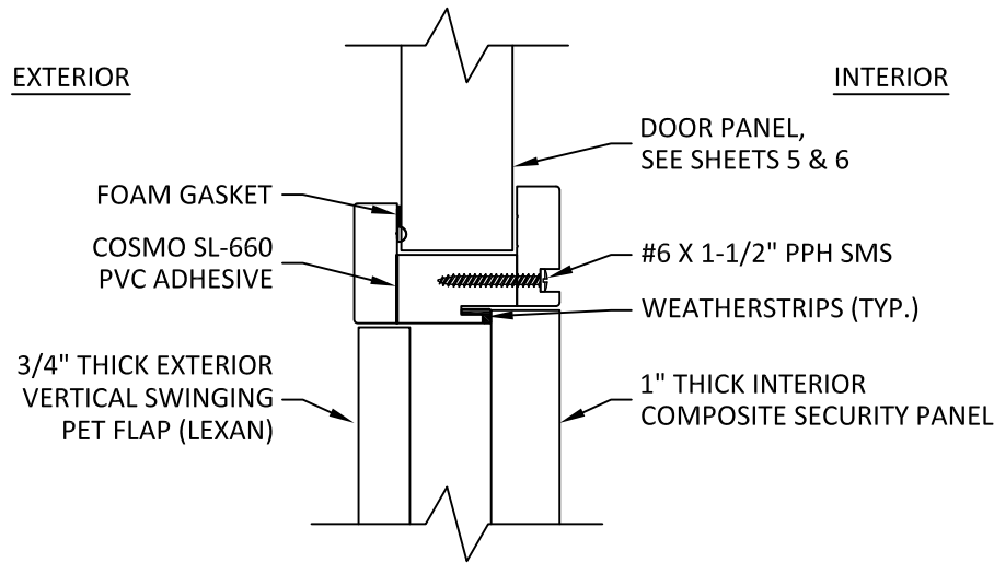
A 4 VERTICAL SECTION PET DOOR HEAD
