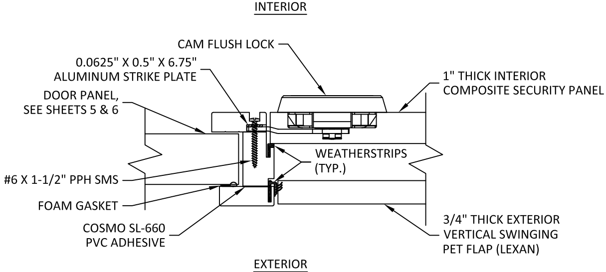
C 4 HORIZONTAL SECTION PET DOOR LOCK JAMB
