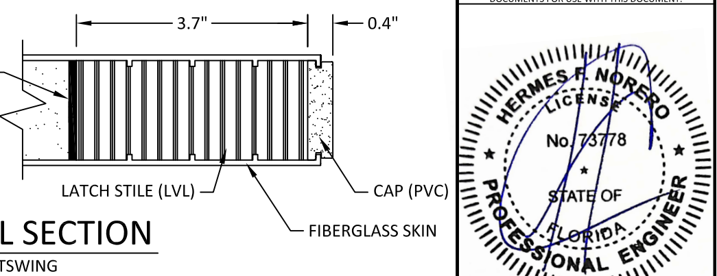
4 6 HORIZONTAL SECTION INSWING/OUTSWING
