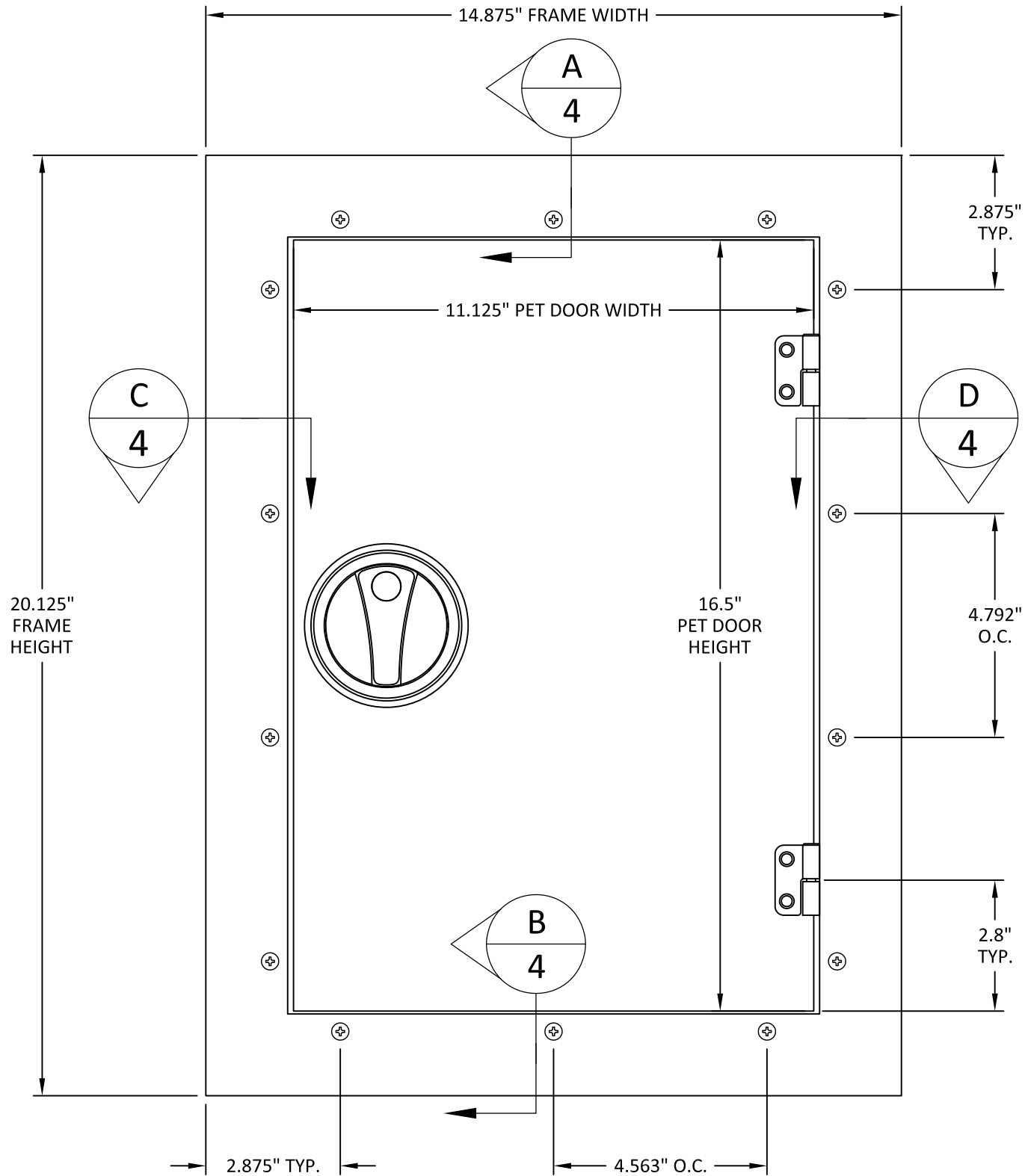
TYPICAL ELEVATION
