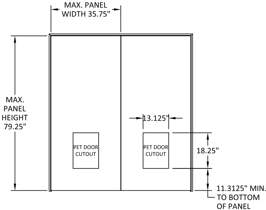
APPROVED CONFIGURATION DOUBLE, 6'-8", INSWING OR OUTSWING
