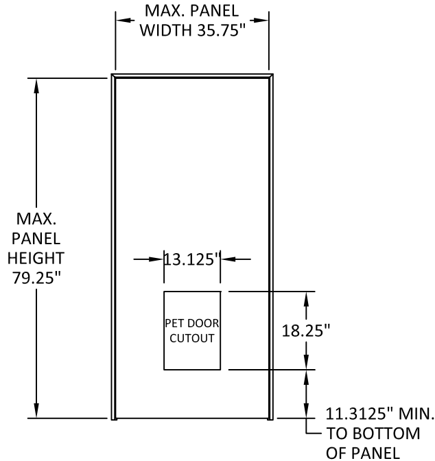
APPROVED CONFIGURATION SINGLE, 6'-8", INSWING OR OUTSWING
