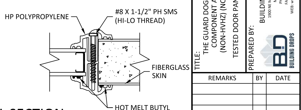
4 6 HORIZONTAL SECTION INSWING/OUTSWING
