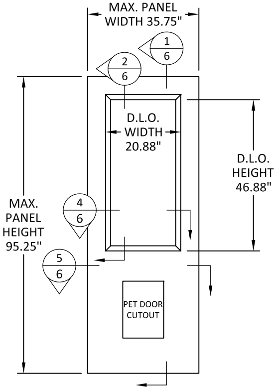
TESTED PANEL GLAZED, 8'-0"
