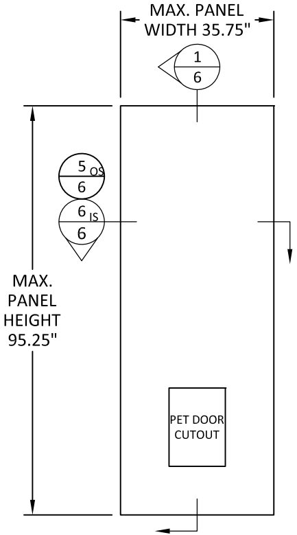
TESTED PANEL OPAQUE, 8'-0"
