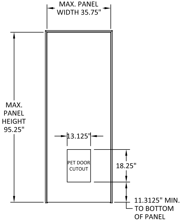
APPROVED CONFIGURATION SINGLE, 8'-0", INSWING OR OUTSWING
