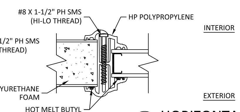
4 6 HORIZONTAL SECTION INSWING/OUTSWING
