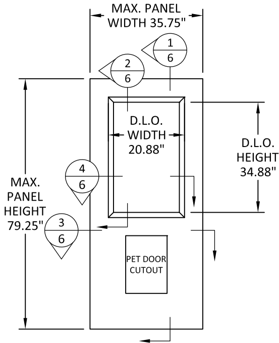
TESTED PANEL GLAZED, 6'-8"
