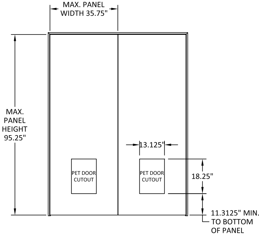
APPROVED CONFIGURATION DOUBLE, 8'-0", INSWING OR OUTSWING
