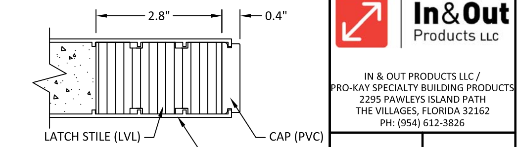
3 6 HORIZONTAL SECTION INSWING/OUTSWING
